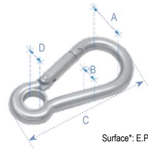
Snap Hook with Eye End, Inox 316
