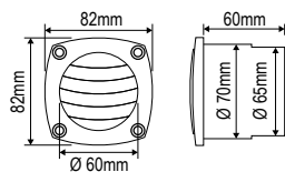
Ventilation Shaft Grilles, White
