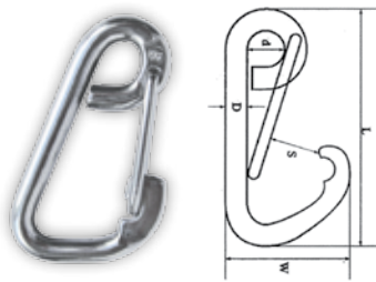
Spring Snap with Angled Latch, Inox 316
