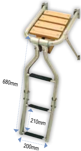
Wooden Platform with Inox 316 Ladder
