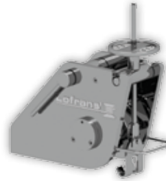
Chain Roller-Stopper with Tensioner, Inox, for ISO/DIN/Studlink Chain 14/16mm
