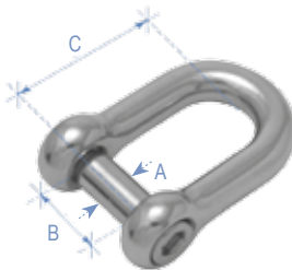
Shackle, Type D, with Inter. Hexagonal Sink Pin, AISI 316
