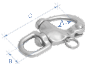
Snap Shackle, with Swivel, Inox 316
