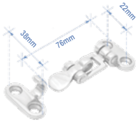
Cover Latch, Inox 316
