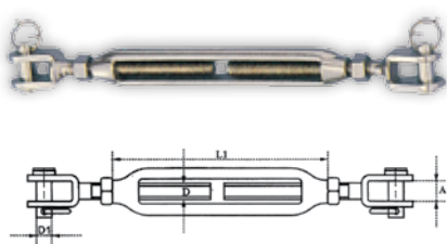
Frame Turnbuckle with Nut, Jaw & Jaw, Inox 316
