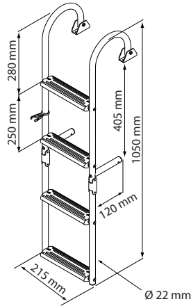
Foldable Ladder for Narrow Transom, 2+2 Steps, Inox 316, 180°
