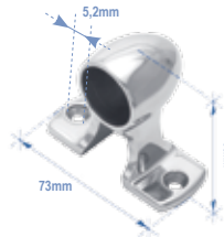
Rail Fitting, Top Side Cap 90°, Inox 316
