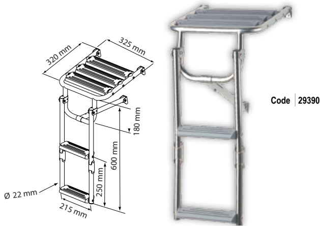
Platform Ladder, Inox 316, with 2 Plastic Steps
