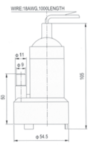
Water Pump for Tanks 160GPH, 12V, 2,5A
