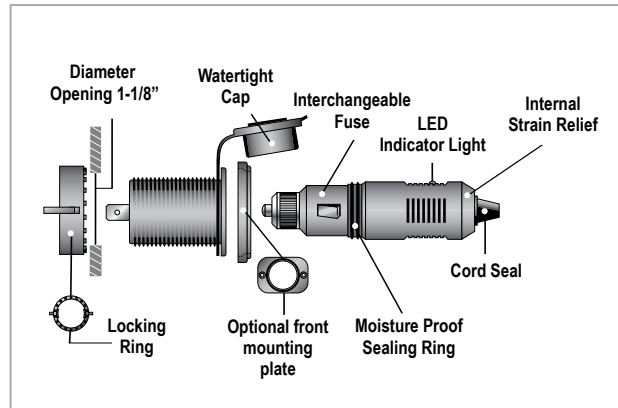
Marine Terminal Socket, 12V
