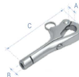
Pelican Hook, Inox 316
