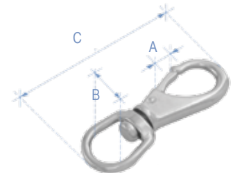
Swivel Eye Snap, Inox 316
