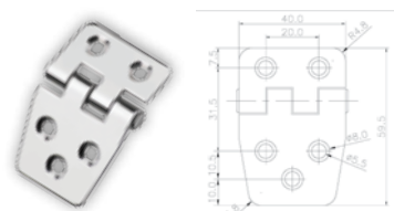
Hinge, Reversed, Inox 316
