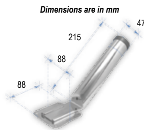
Fishing Rod Holder, Removable, Inox 304
