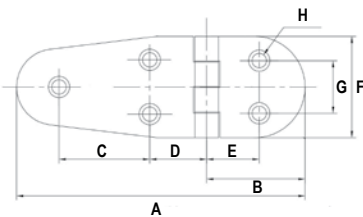
Hinge, Right, Inox 316
