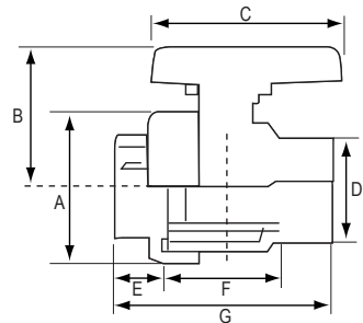
Ball Valve, Single Union BSPT, Plastic, with Blue Handle
