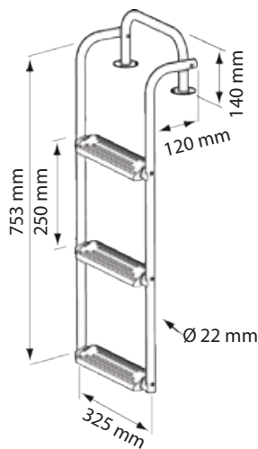
Bow Ladder, 3 Steps, Inox 316
