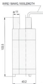
Water Pump for Tanks 100GPH, 12V, 2A
