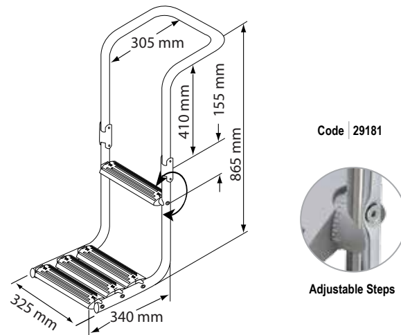
Immersed Platform Ladder, Inox 316
