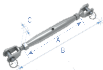
Pipe Turnbuckle with Nut, Jaw & Jaw, Inox 316
