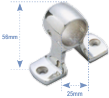
Fitting for Rails, Central Cap 90°, Inox 316
