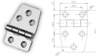
Hinge, Right, Inox 316
