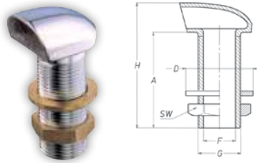
Fuel Tank Vent 5/8" I.D. Hose Die Cast Zamak, 16cm
