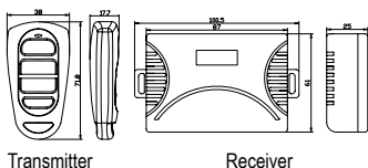
Transmitter
