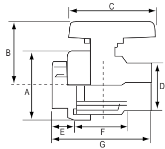
Ball Valve, Single Union, BSPP, Plastic, with Orange Handle
