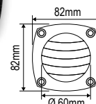
Ventilation Shaft Grilles Cover, PA
