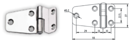
Hinge, Right with Angle, Inox 316
